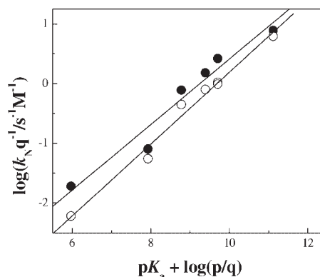
Figure 1. Brønsted-type plots (statistically corrected, see text) for the reactions of SA amines with PNPTC (O) and CIPNPTC (●) in 44 wt% ethanol–water, at 25.0°C, ionic strength 0.2 M (KCl)
