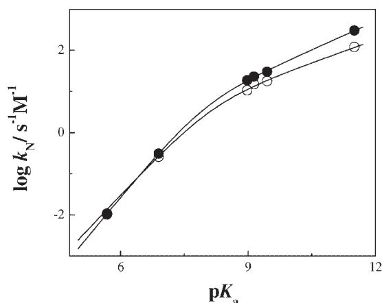
Figure 2. Brønsted-type plots for the reactions of pyridines with PNPTC (O) and CIPNPTC (●) in 44 wt% ethanol–water, at 25.0°C, ionic strength 0.2 M (KCl)
